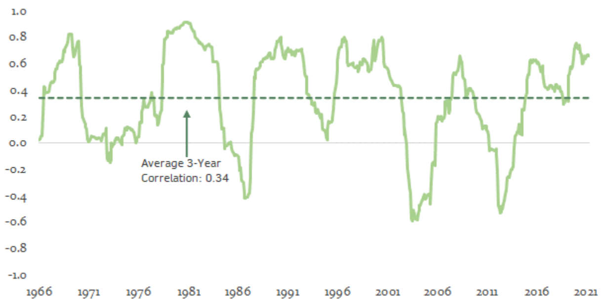
Figure 1: Momentum and Growth Rolling Correlations
