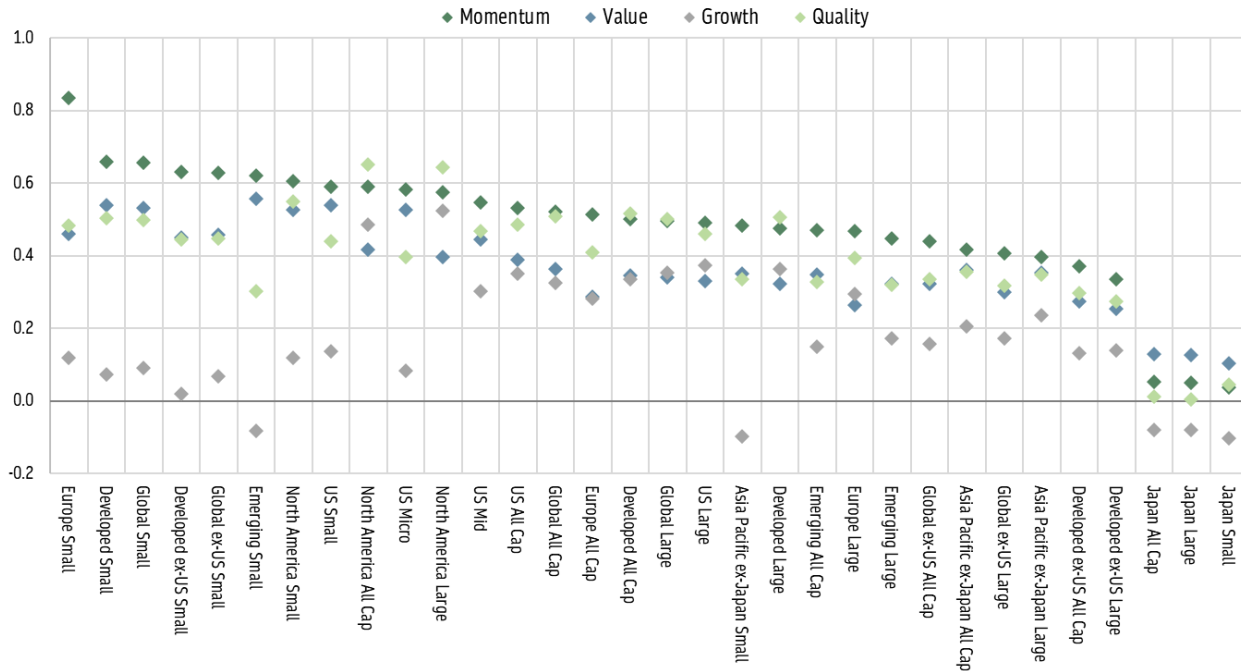
Figure 1: Sharpe Ratios
